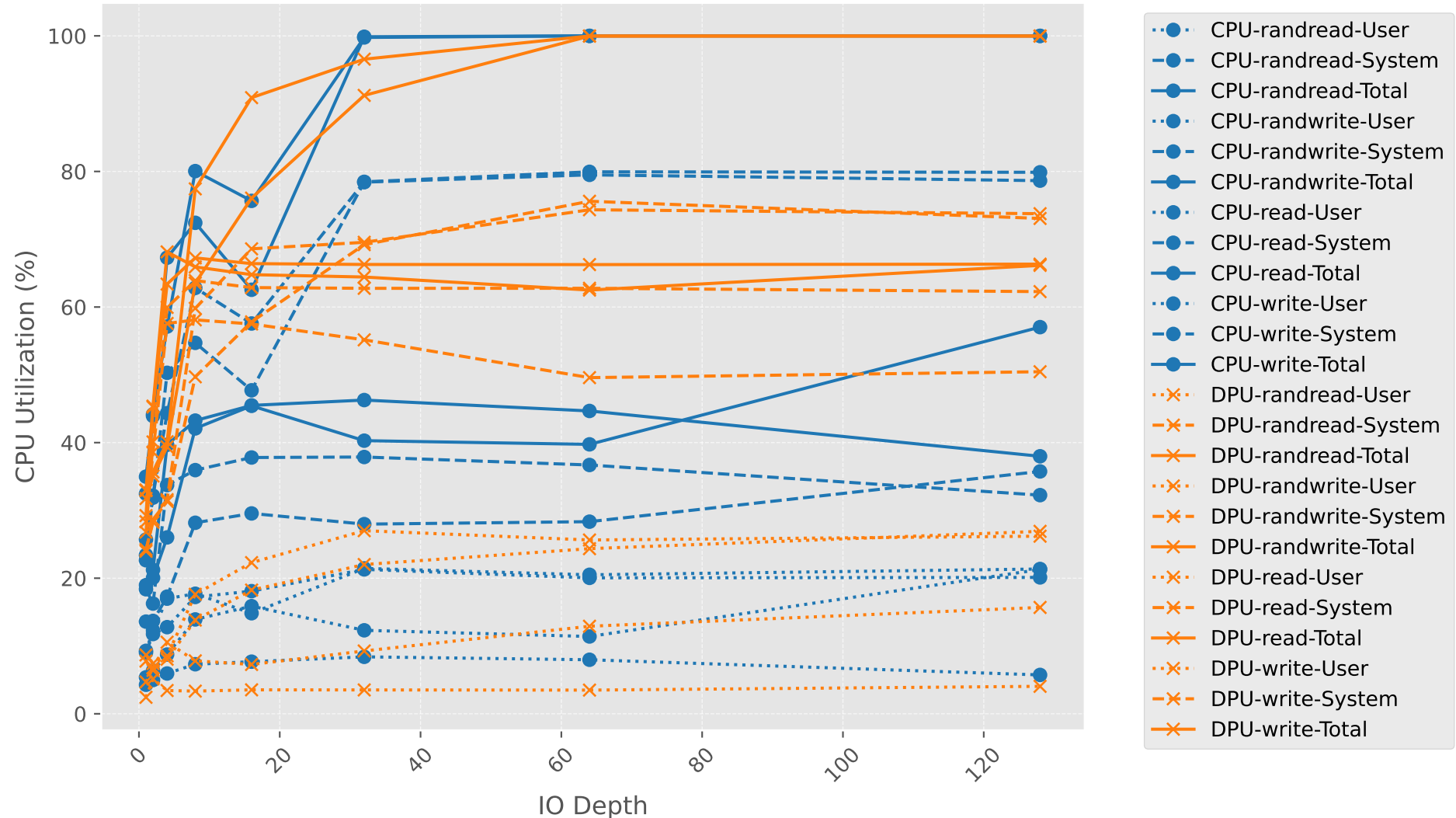
CPU Total vs IO Depth
